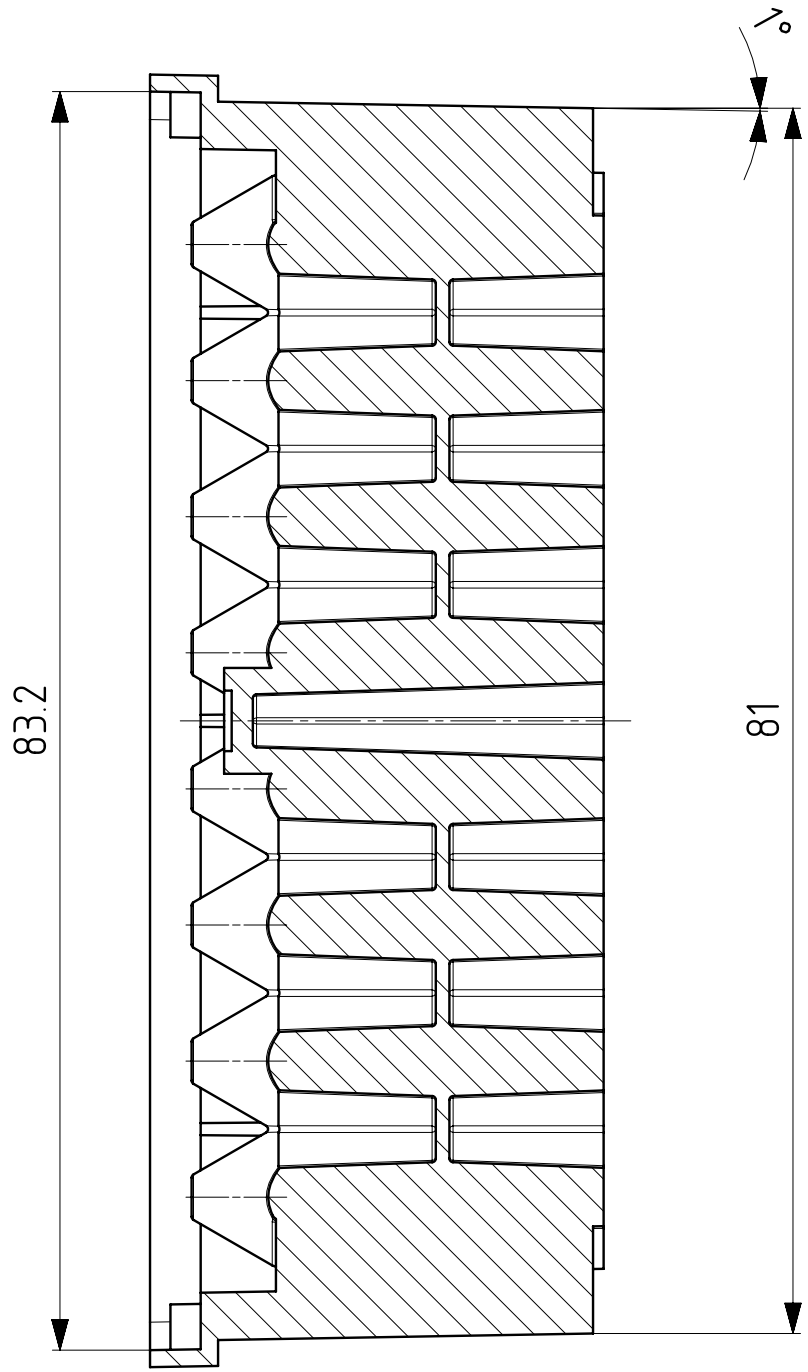
SECTION B-B
